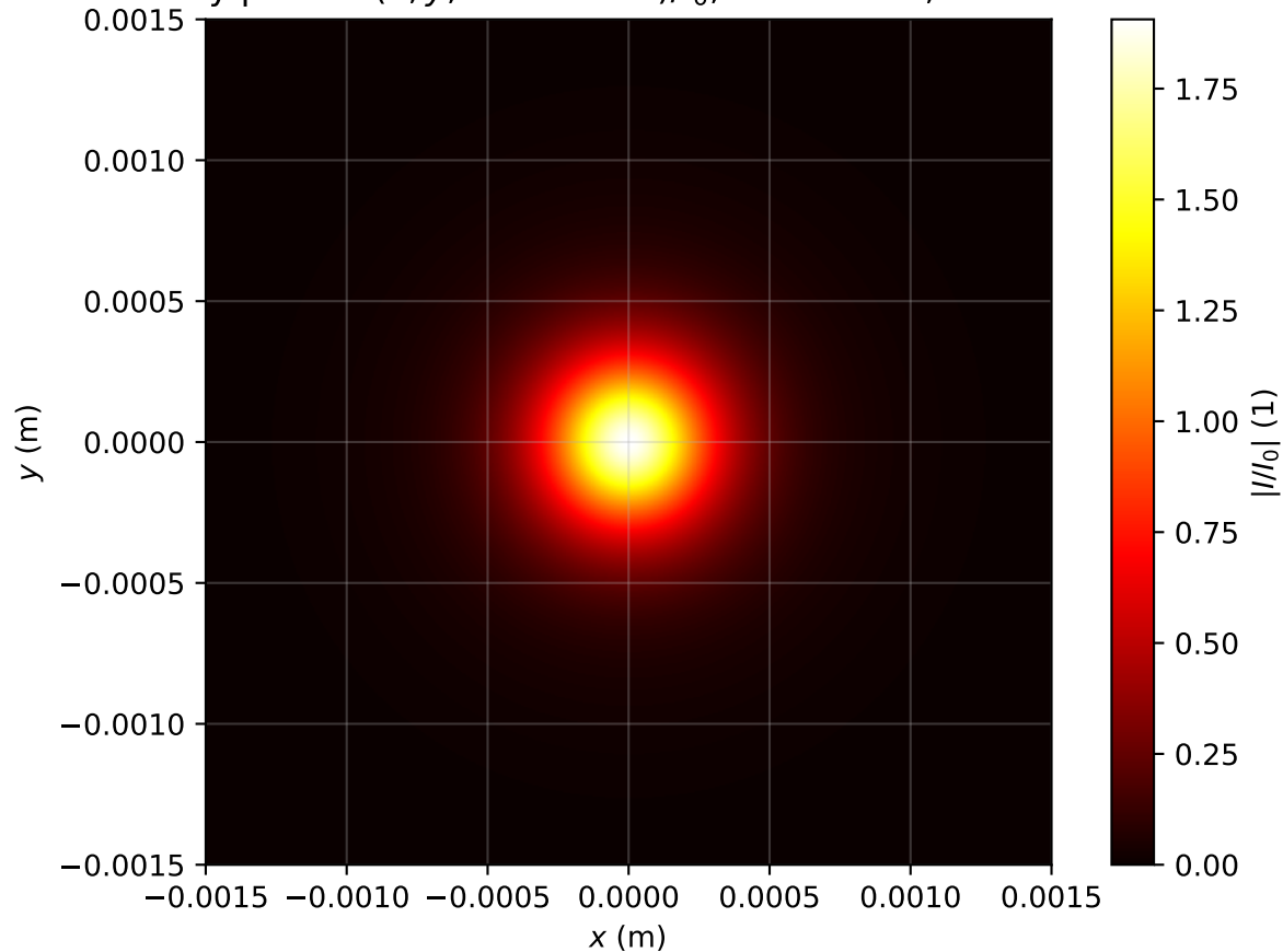
Intensity profile I(x, y, z = 1.592m)/I_0 , P_{in}=1.0P_{cr} , artificial time
